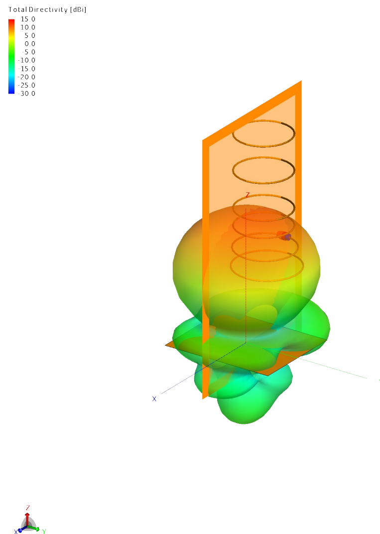
Figure 2: 3D View
