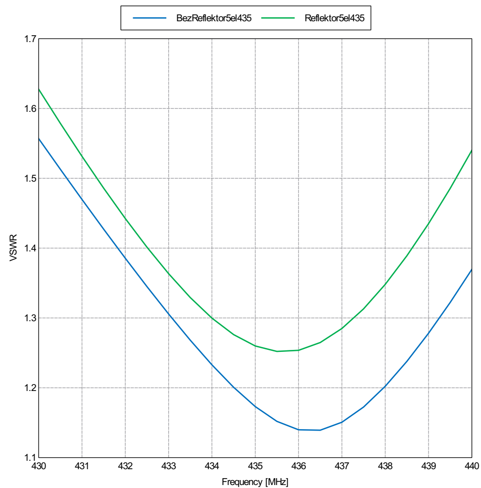
Figure 3: VSWR
