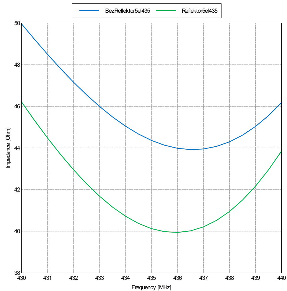
Figure 4: Impedance Magnitude
