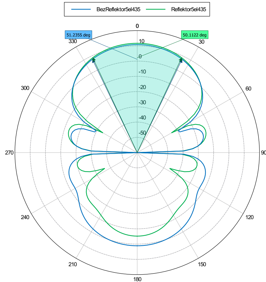
Figure 5: Theta Directivity (Frequency = 435 MHz; Phi = 90 deg)
