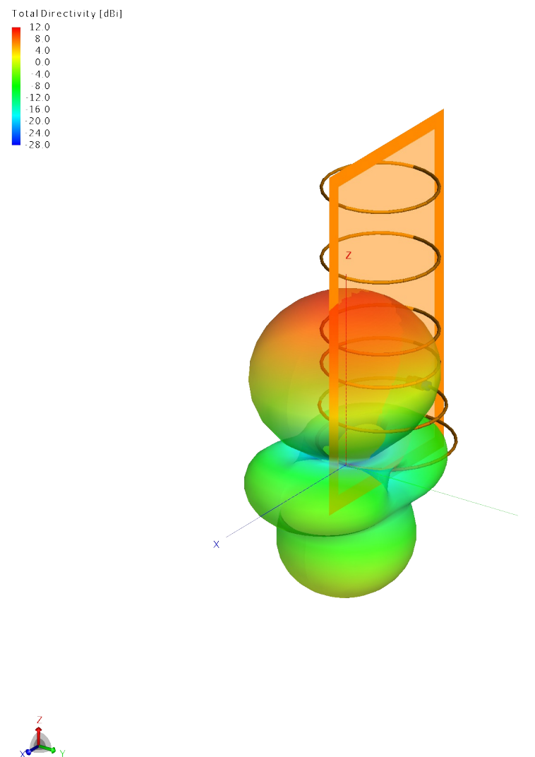
Figure 1: 3D View
