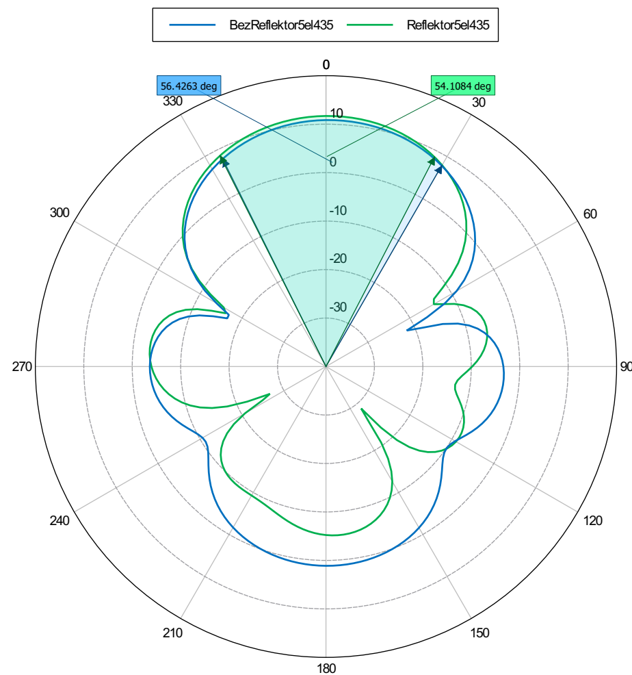
Figure 6: Phi Directivity (Frequency = 435 MHz; Phi = 0 deg)
