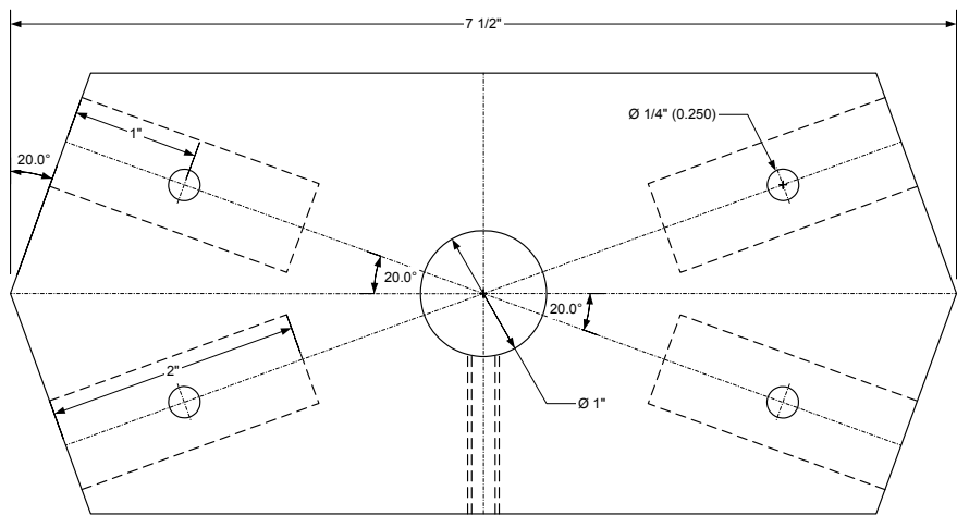
TOP VIEW
