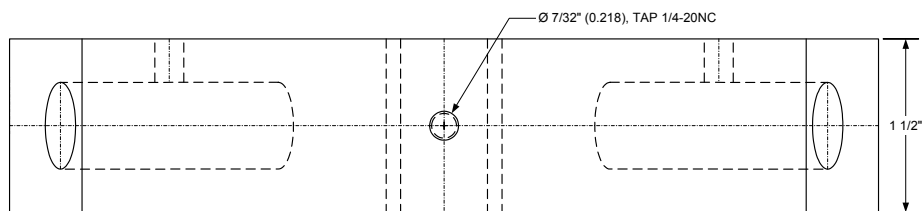
FRONT VIEW
