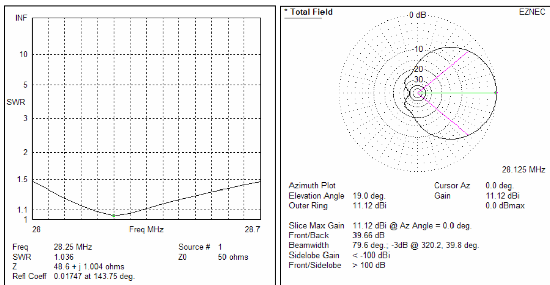
Figure 2 10-Meter MoxBeam SWR and Azimuth plots @ 25 feet
